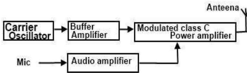
Figure (b) Block diagram of Low-level AM transmitter
